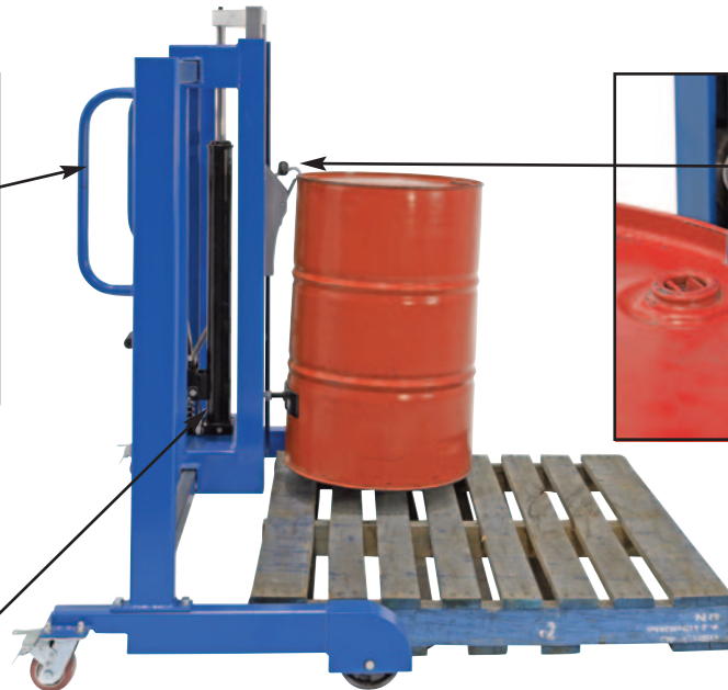
Spring loaded clamp to securely hold the drum
